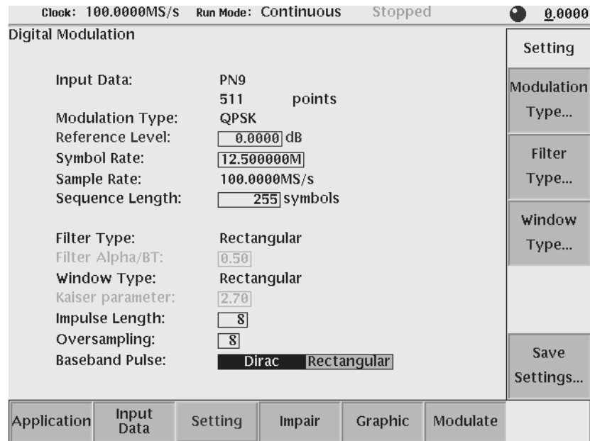
Figure 3-52: Setting menu
