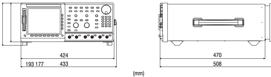
Figure A-4: Dimensions
