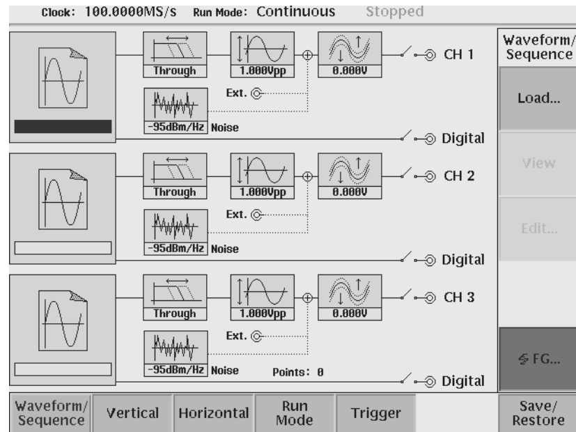
Figure 2-34: Initial screen
