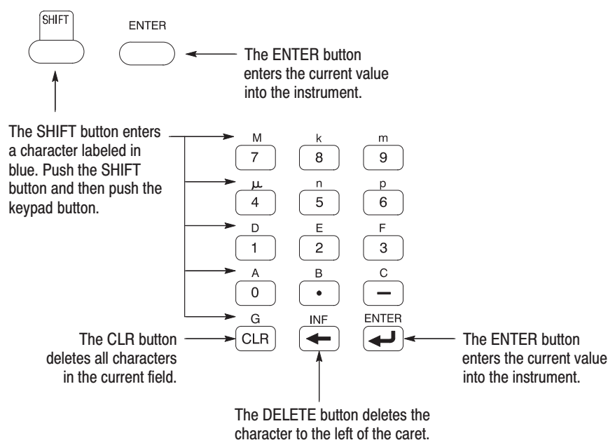
Figure 2-11: Keypad buttons
