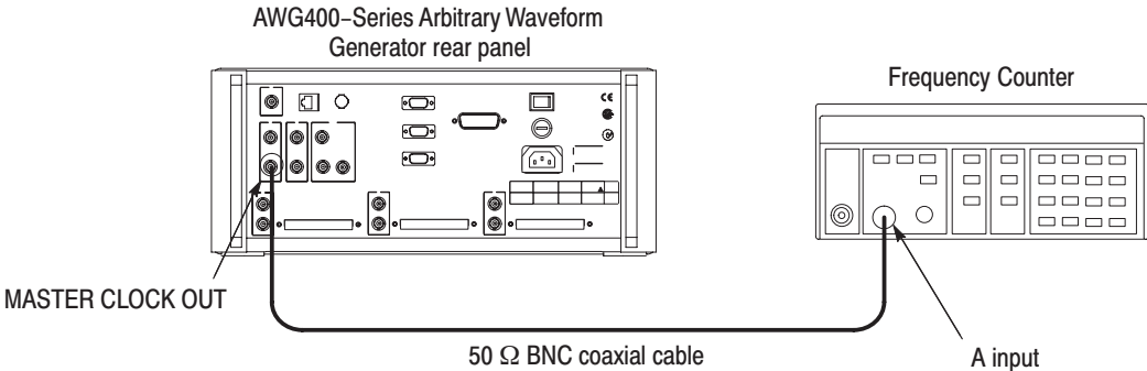
Figure B-14: Clock frequency and 10 MHz reference input initial test hookup
