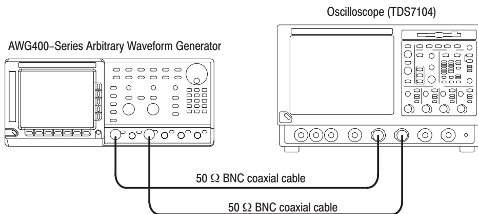
Figure B-42: Channel skew test hookup
